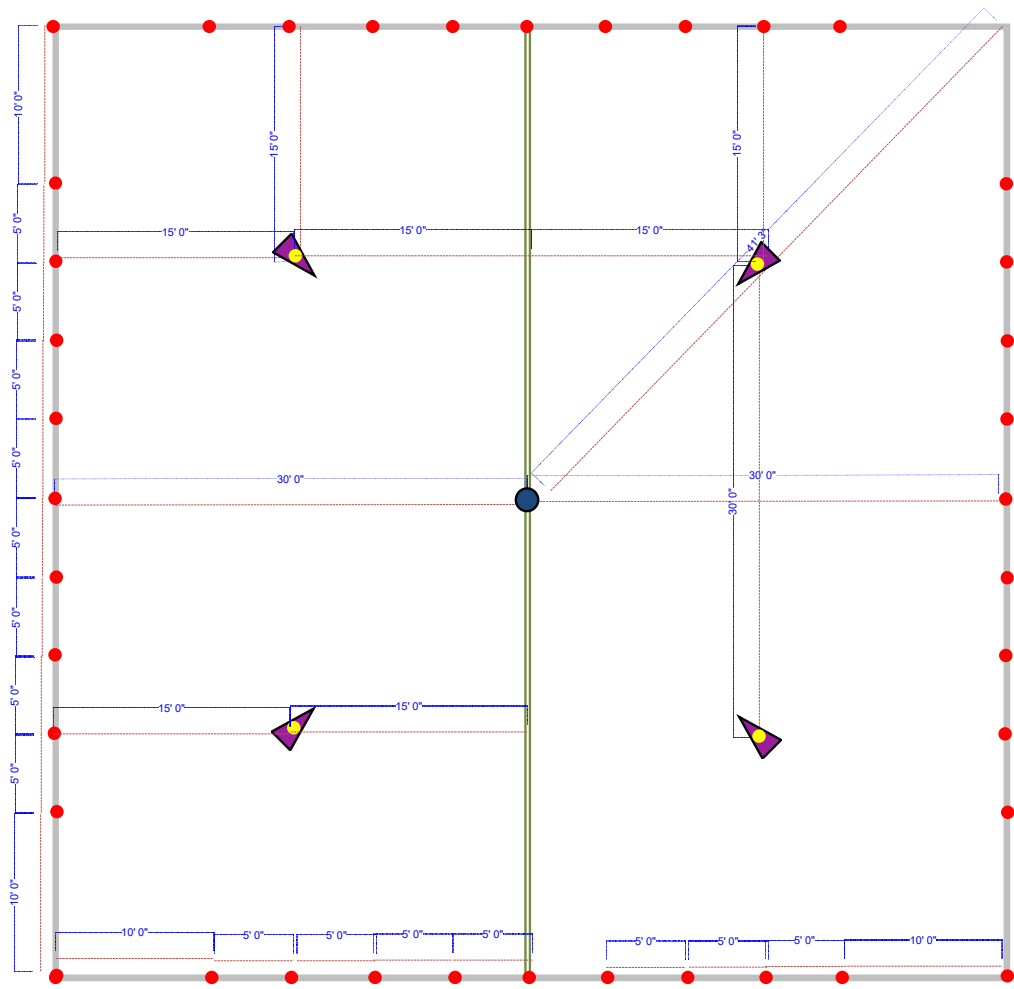
60' x 60' Pole Tent - Pole Placements
